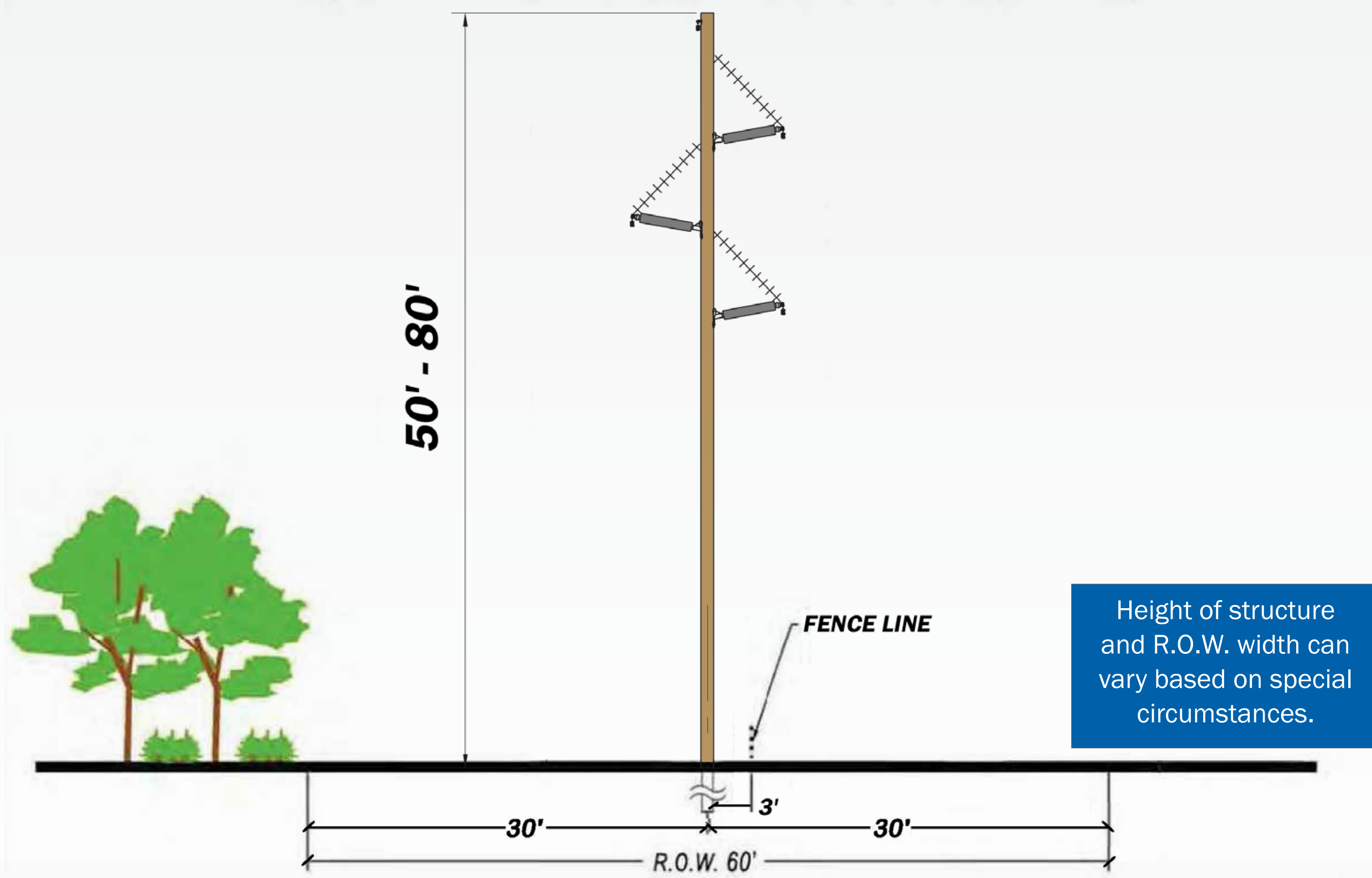
Typical 115kV Single Circuit, Single Pole Structure
