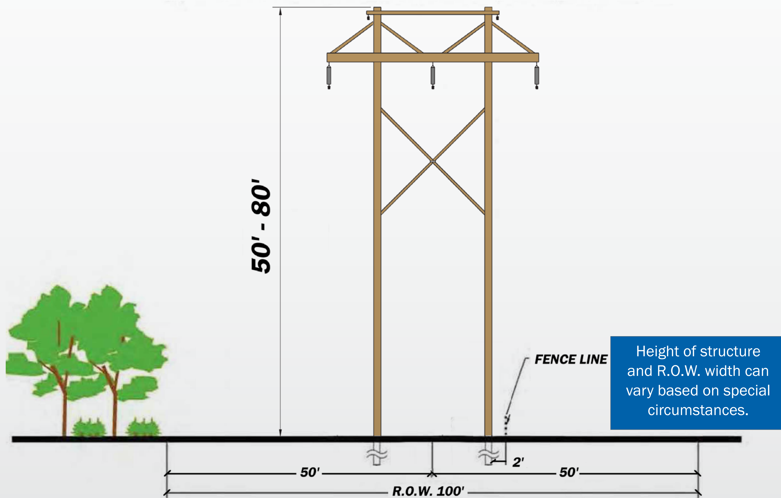
Typical 115kV Single Circuit, Two-Pole Structure
